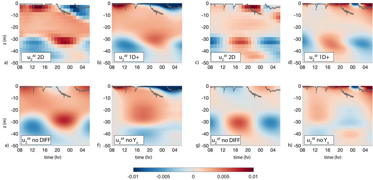
FIG. 6. (left),(left center) Alongfront and (right center),(right) cross-frontal shear predicted by (a),(c) 2D, (b),(d) 1D+, (e),(g) 1D+ without friction (no DIFF), and (f),(h) 1D+ without initial shear (no Y_o ). Float depth from OBS (gray dots) is included for reference.
