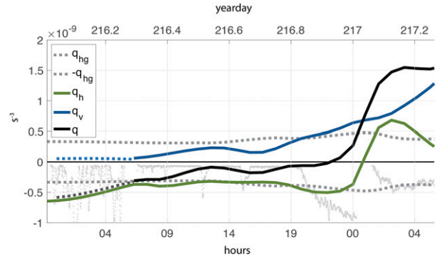
FIG. 9. The PV at 8 m from 2D using N_{ADV}^2 to isolate changes resulting from vertical shear: total q (black), horizontal q_h (green) and vertical q_v (blue). Gray dashed lines are the PV associated with thermal wind balance q_{hg} = -b_{xt}^2/f . The observed float depth (scaled by a factor of 10^{-10} ) is included for reference.
