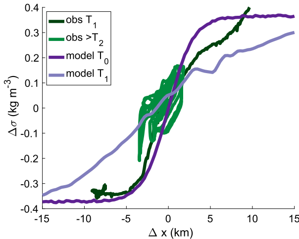
FIG. 4. Cross-frontal density structure from OBS compared with 2D. The initial Triaxus transect (obs T_1 ; dark green) crossed the entire front. Triaxus while following the float (obs > T_2 ; light green) surveyed the sharpest part of the front. Also shown are 2D after one time step, 6 days before OBS (model T_0 ; dark purple), and the cross-frontal structure in 2D at the start of the Lagrangian survey (model T_1 ; light purple) after 6 days of wind forcing.
