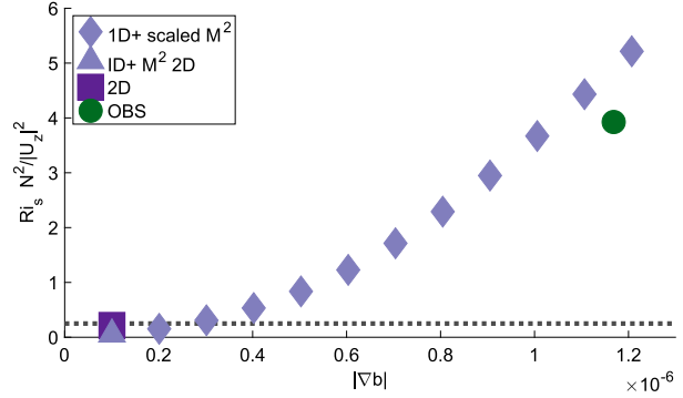
FIG. 12. Comparison between shear Richardson number Ri_s and horizontal buoyancy gradient |\nabla b_h| . The Ri_s was calculated during stage 3 (nighttime mixing) from OBS (green), from 2D (dark purple), and from the solution to 1D+ for varying M^2 (light purple). The dashed gray line corresponds to critical Ri_s = 0.25 .
